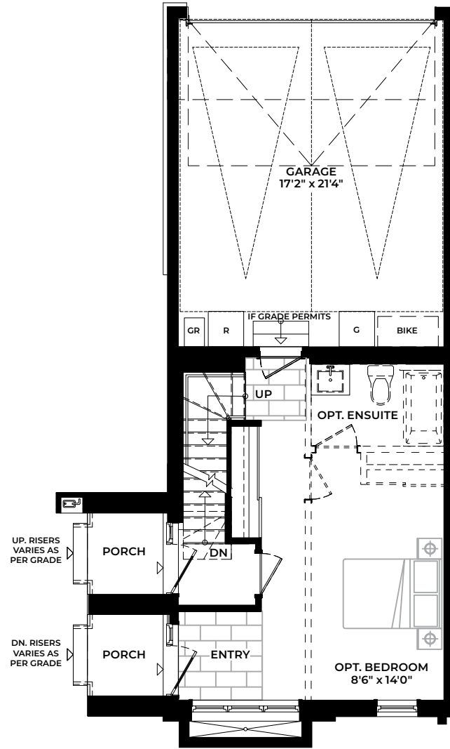
T1 Corner GROUND FLOOR
