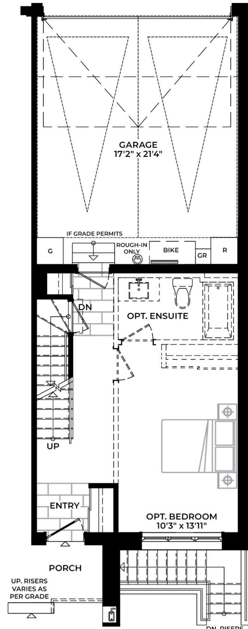
T1 B1 End GROUND FLOOR
