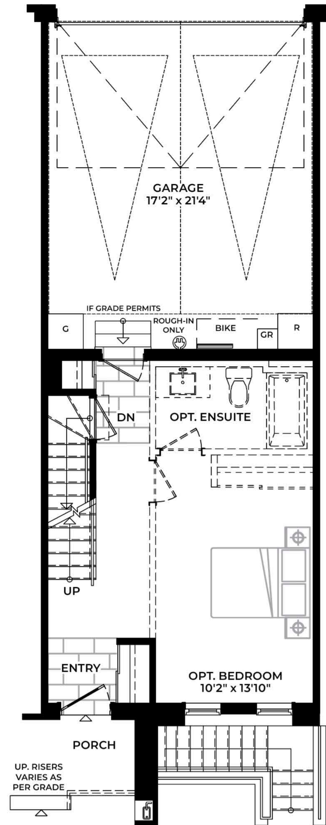
T1 Int. GROUND FLOOR
