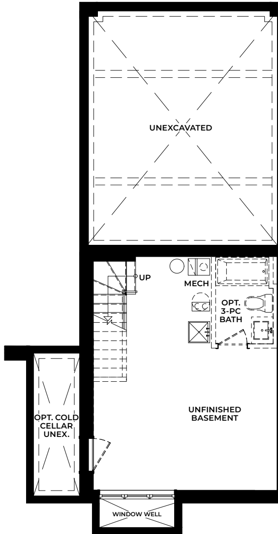
T1 Corner Separate Entrance BASEMENT
